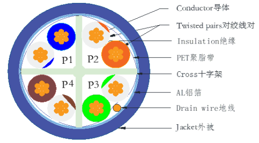
CAT6 F/UTP 4P*26AWG(7/0.16BC,HDPE 0.82mm+CROSS+PET+AL+D) PVC JACKET OD:6.0
