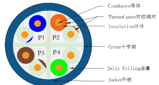
CAT6 U/UTP 4P*23AWG(1/0.57BC,HDPE 1.03mm +CROSS+JELLY) PVC JACKET OD:6.3
