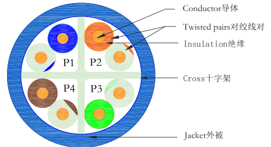
CAT6 U/UTP 4P*23AWG(1/0.57CCA,HDPE 1.03mm +CROSS) PVC JACKET OD:6.3
