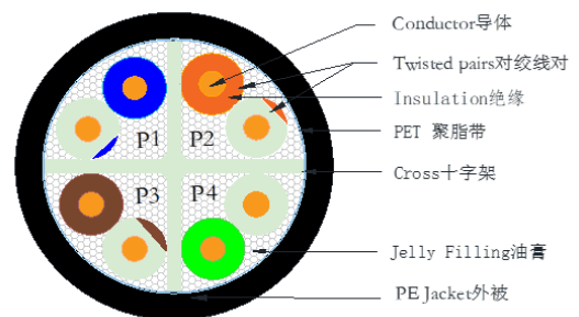
CAT6 U/UTP 4P*23AWG(1/0.57BC,HDPE 1.03mm +CROSS+PET+JELLY) PVC JACKET OD:6.3
