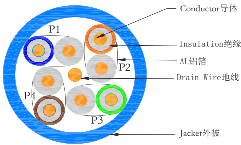
CAT6A U/FTP 4P*23AWG(1/0.58BC,FM-PE 1.42mm+AL+D) LSZH JACKET OD:7.8
