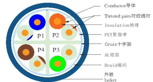
CAT6A SF/UTP 4P*23AWG(1/0.57BC,HDPE 1.1mm +CROSS+PET+AL+B) PVC JACKET OD:7.7
