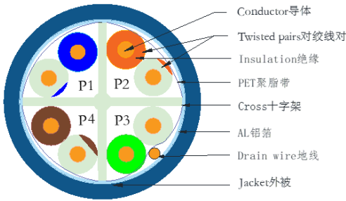
CAT6A F/UTP 4P*23AWG(1/0.57BC,HDPE 1.1mm +CROSS+PET+AL+D) PVC JACKET OD:7.7
