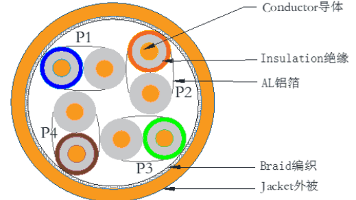
CAT7 S/FTP 4P*23AWG(1/0.58BC,FM-PE 1.42mm+AL+B) LSZH JACKET OD:7.8
