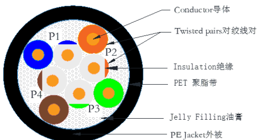
CAT5e U/UTP 4P*24AWG(1/0.5BC,HDPE 0.88mm +PET+JELLY) PVC JACKET OD:5.2
