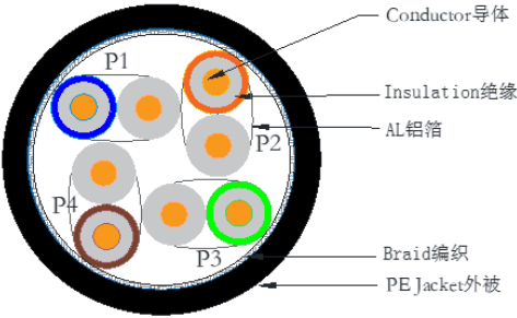
CAT7 S/FTP 4P*23AWG(1/0.58BC,FM-PE 1.42mm+AL+D+B) PE JACKET OD:7.8
