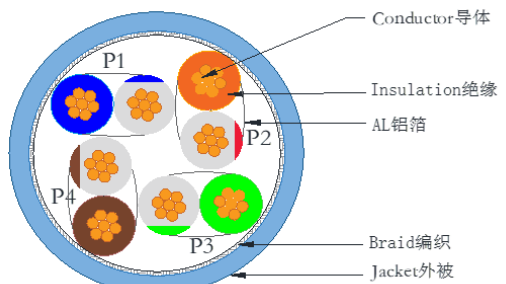
CAT8 S/FTP 4P*26AWG(7/0.16BC,FM-PE 1.08mm+AL +B) LSZH JACKET OD:6.5
