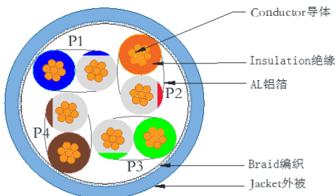
CAT7 S/FTP 4P*26AWG(7/0.16BC,FM-PE 1.08mm+AL +B) LSZH JACKET OD:6.2
