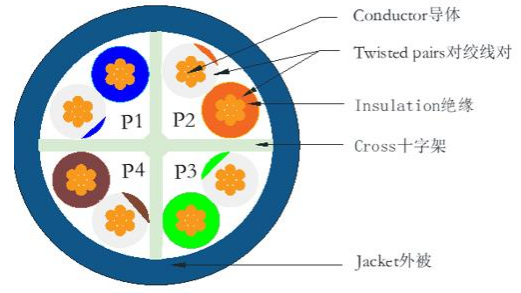
CAT6 UTP 4P*26AWG(7/0.16BC,HDPE 0.77mm) PVC JACKET OD:6.0
