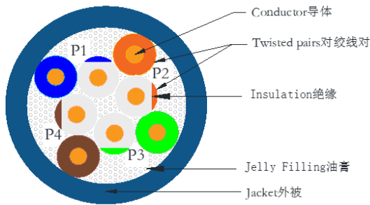
CAT5e U/UTP 4P*24AWG(1/0.5BC,HDPE 0.88mm +JELLY) PVC JACKET OD:5.2
